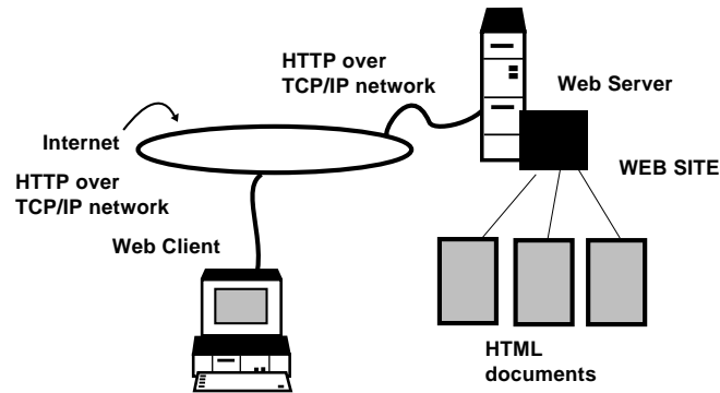
Figure 1-8: Traditional file-based web site
