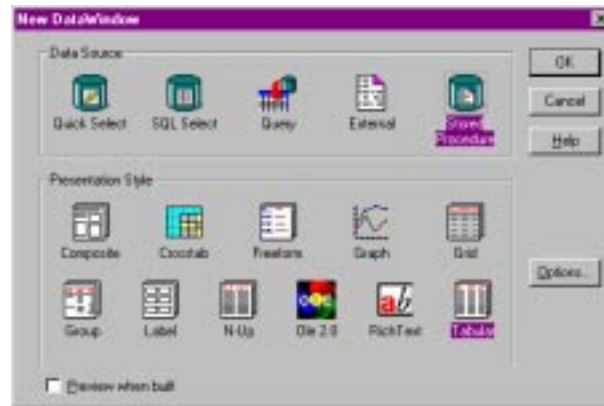
Figure 3-5: PowerBuilder development window
