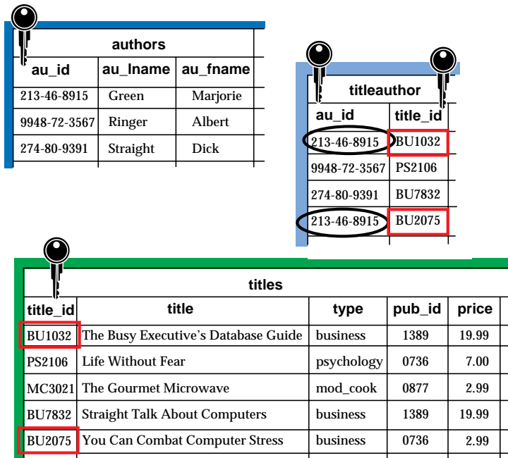
Figure 1-2: Retrieving data across tables using key columns
