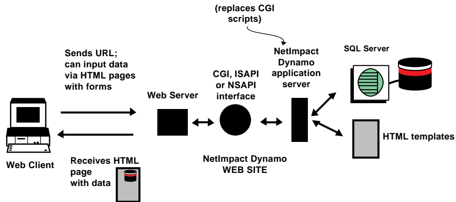
Figure 1-9: How NetImpact Dynamo interacts with SQL Server and the web server
